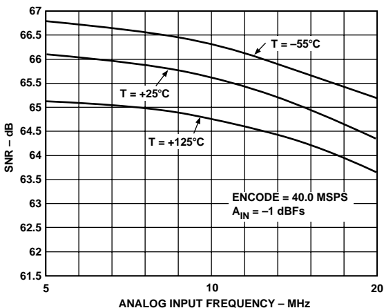
Figure 12. SNR vs. A_{IN}
