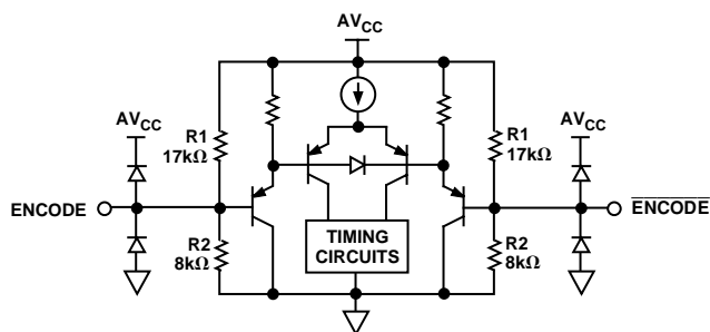
Figure 4. Encode Inputs
