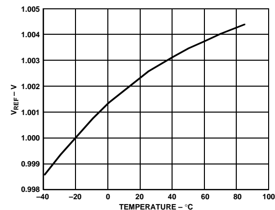
Figure 9. Voltage Reference Error vs. Temperature
