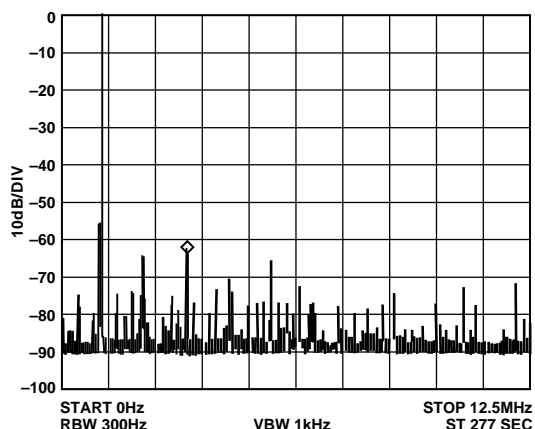
Figure 12. f_{MCLK} = 25 MHz, f_{OUT} = 1.1 MHz, Frequency Word = B439581
