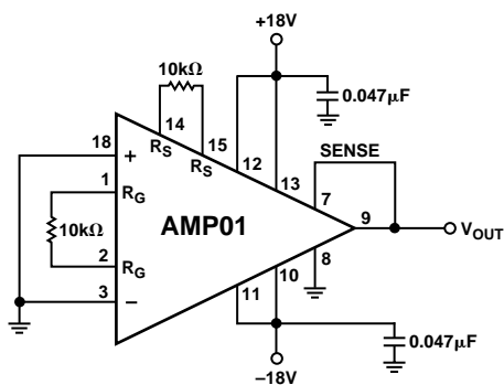
Figure 47. Burn-In Circuit
