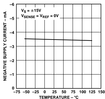
Figure 28. Negative Supply Current vs. Temperature
