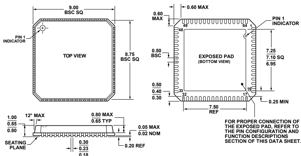
Figure 10. 64-Lead Lead Frame Chip Scale Package [LFCSP_VQ] 9 mm x 9 mm Body, Very Thin Quad (CP-64-3) Dimensions shown in millimeters
