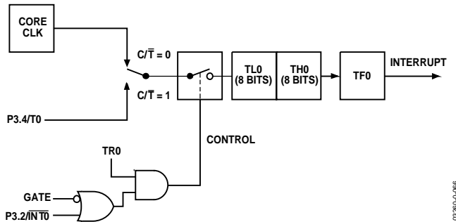
Figure 67. Timer/Counter 0, Mode 1
