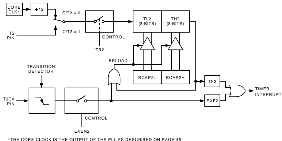
Figure 48. Timer/Counter 2, 16-Bit Autoreload Mode
