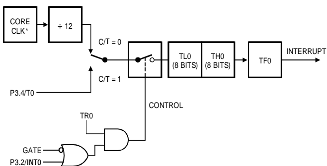
Figure 45. Timer/Counter 0, Mode 1
