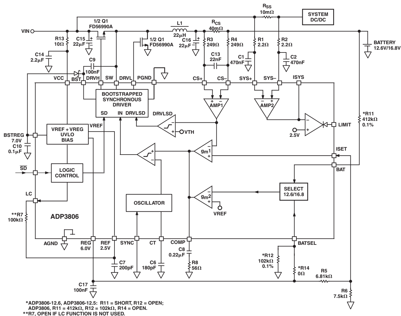
Figure 1. Typical Application
