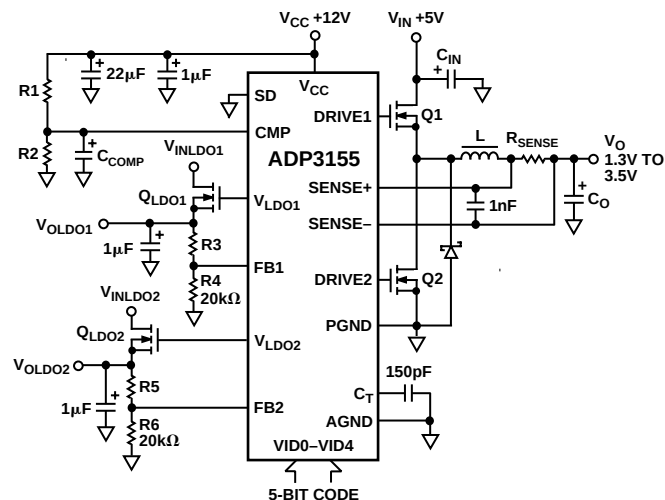
Figure 1. Typical Application
