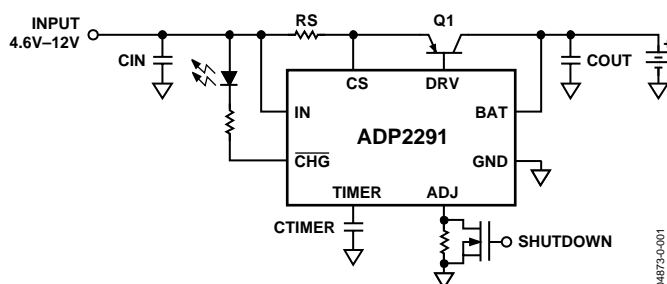
Figure 1. Basic Circuit Configuration
