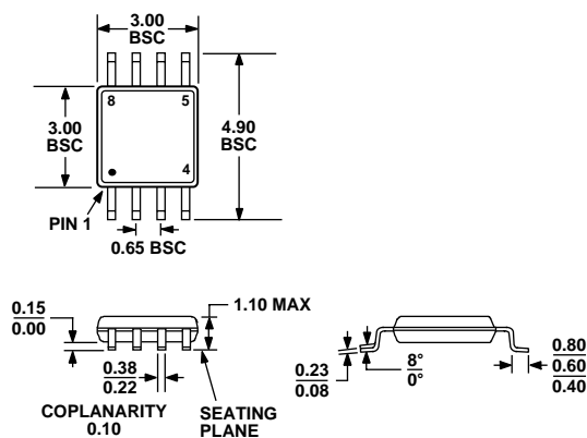
Figure 29. 8-Lead MSOP Package (RM-8)
