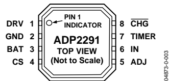
Figure 3. 8-Lead LFCSP
