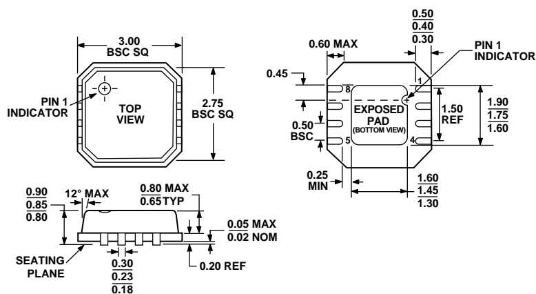
Figure 28. 8-lead 3 × 3 LFCSP Package (CP-8)
