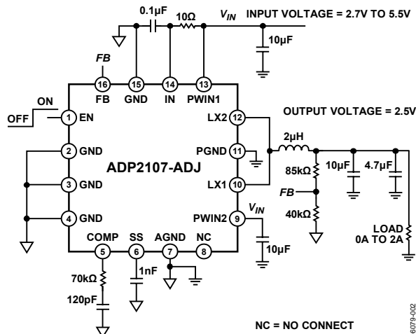
Figure 2. Circuit Configuration of ADP2107 with V_{OUT} = 2.5 V
