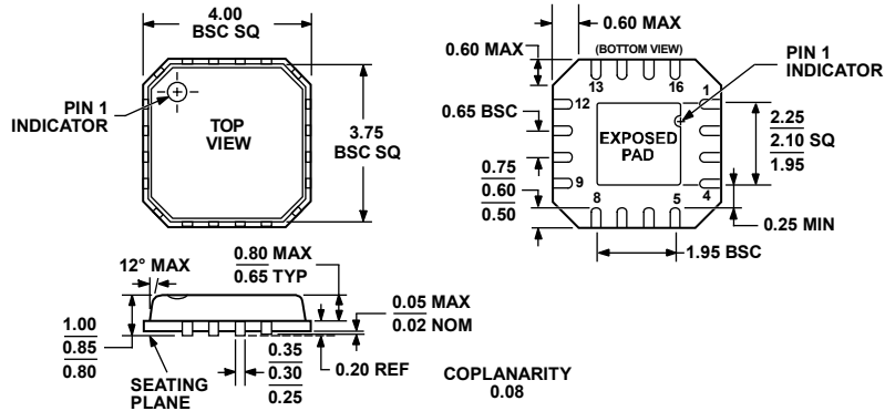
Figure 61. 16-Lead Lead Frame Chip Scale Package [LFCSP_VQ] 4 mm × 4 mm Body, Very Thin Quad (CP-16-4)
