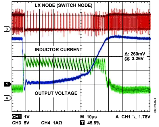
Figure 25. Short Circuit Response at Output
