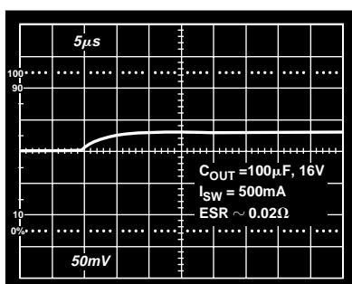
Figure 14. OS-CON Capacitor
