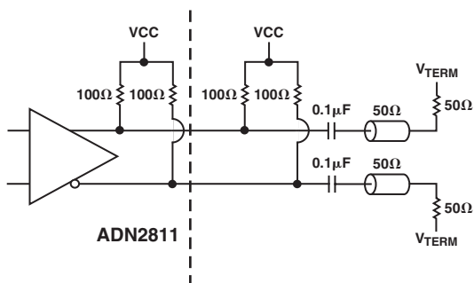
Figure 18. AC-Coupled Output Configuration
