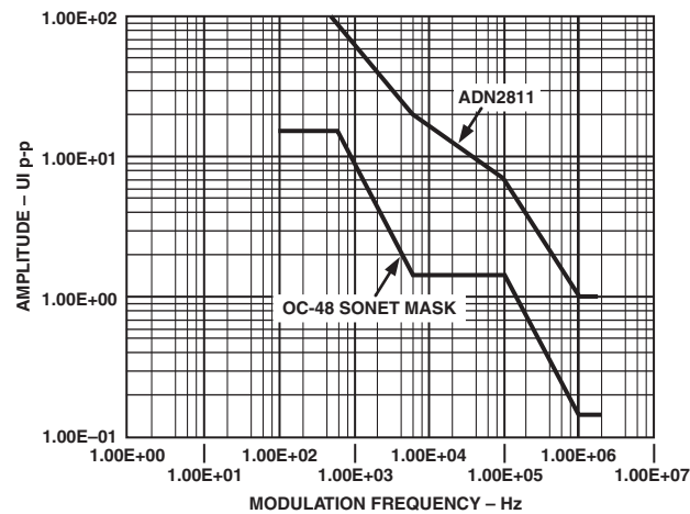
Figure 9. OC-48 Jitter Tolerance Curve
