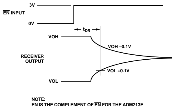
Figure 22. Receiver-Disable Timing
