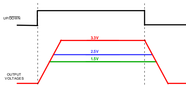
Figure 1. ADM1200-1 Power-Up and Power-Down Waveforms
