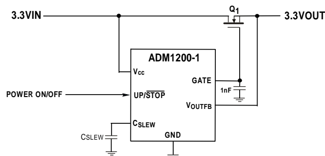
Figure 3. ADM1200 Switching on a Single Supply
