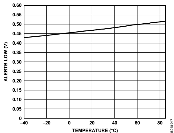
Figure 30. Output Low Voltage vs. Temperature @ 1 mA
