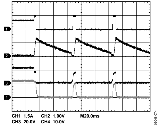
Figure 48. Overcurrent Condition During Operation (ADM1178-2 Model) (CH1 = I_{LOAD} , CH2 = V_{TIMER} , CH3 = V_{GATE} , CH4 = V_{OUT} )
