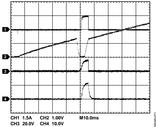
Figure 45. Overcurrent Condition at Startup (ADM1178-1 Model) (CH1 = I_{LOAD} , CH2 = V_{TIMER} , CH3 = V_{GATE} , CH4 = V_{OUT} )
