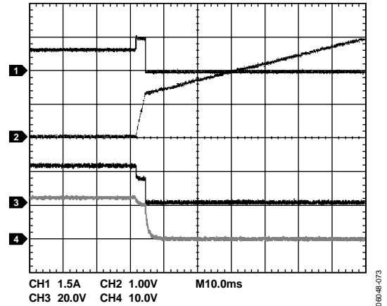
Figure 47. Overcurrent Condition During Operation (ADM1178-1 Model) (CH1 = I_{LOAD} , CH2 = V_{TIMER} , CH3 = V_{GATE} , CH4 = V_{OUT} )
