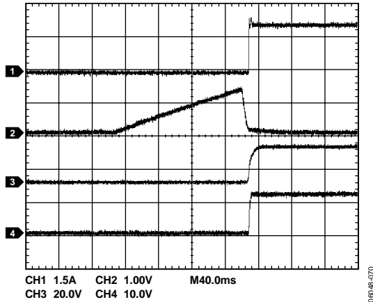
Figure 44. Inrush Current Control into 220 \mu F Load (CH1 = I_{LOAD} , CH2 = V_{TIMER} , CH3 = V_{GATE} , CH4 = V_{OUT} )
