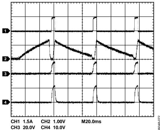
Figure 46. Overcurrent Condition at Startup (ADM1178-2 Model) (CH1 = I_{LOAD} , CH2 = V_{TIMER} , CH3 = V_{GATE} , CH4 = V_{OUT} )
