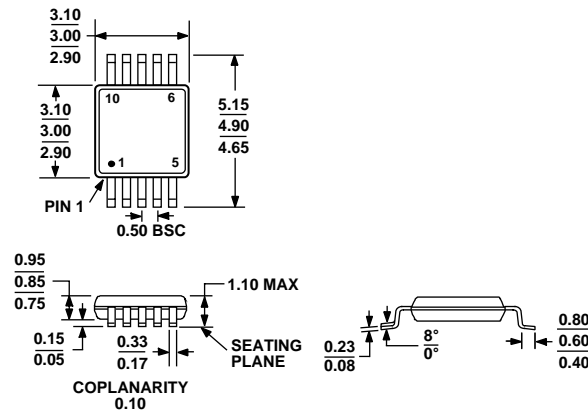
COMPLIANT TO JEDEC STANDARDS MO-187-BA Figure 50. 10-Lead Mini Small Outline Package [MSOP] (RM-10) Dimensions shown in millimeters
