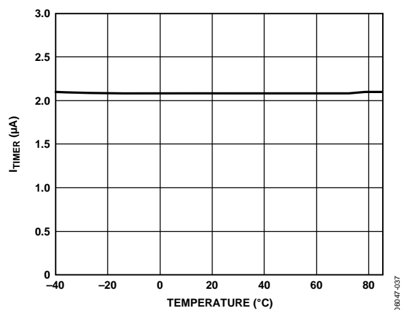
Figure 21. Timer Pull-Down Current (Cool-Off Cycle) vs. Temperature
