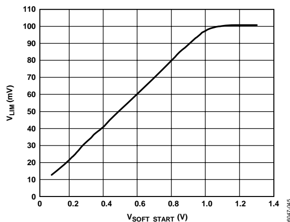
Figure 31. V_{\text{LIM}} vs. V_{\text{SS}}
