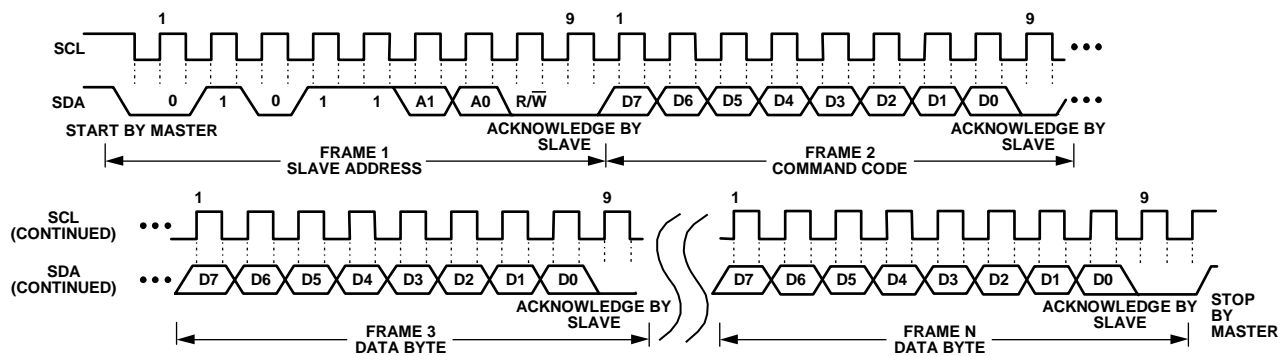
Figure 32. General I²C Write Timing Diagram
