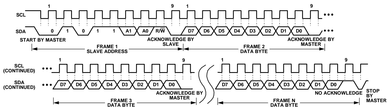
Figure 33. General I²C Read Timing Diagram
