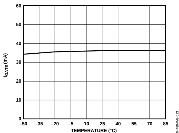
Figure 13. I_{GATE} (FCL, Sink) vs. Temperature ( V_{GATE} = 2\text{ V} )
