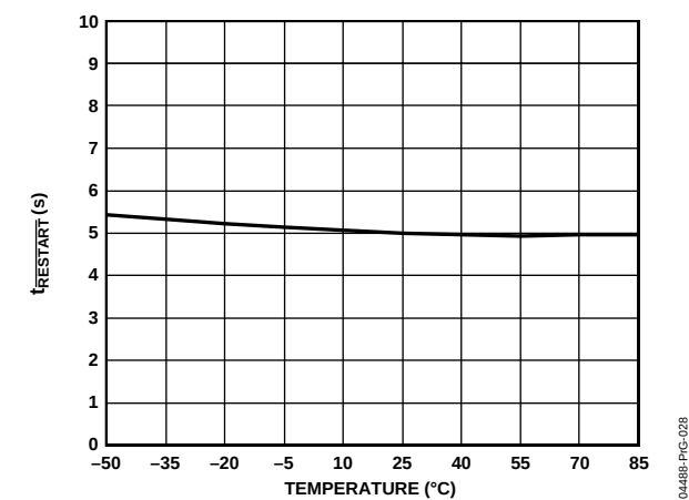
Figure 28. \overline{RESTART} Time vs. Temperature
