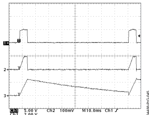
Figure 45. Timing Waveforms during a Retry Cycle for C_{\text{TIMER}} = 0.82 \text{ nF} (Ch1 = GATE; Ch2 = SENSE; Ch3 = \text{TIMER} )
