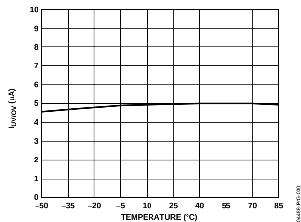
Figure 30. I_{UV/OV} vs. Temperature
