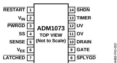
Figure 2. Pin Configuration
