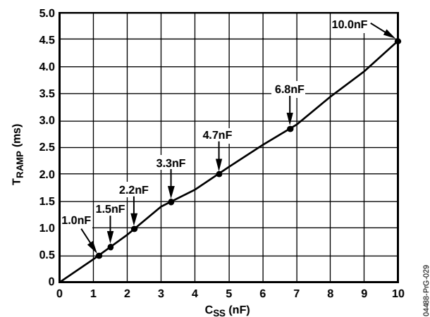
Figure 29. Soft Start Ramp Time vs. C_{SS}
