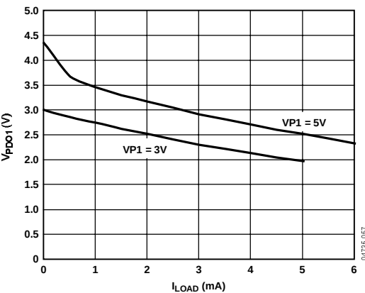
Figure 11. V PDO1 (Strong Pull-Up VP) vs. I LOAD
