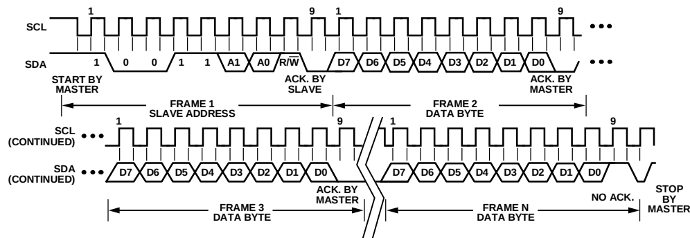
Figure 36. General SMBus Read Timing Diagram
