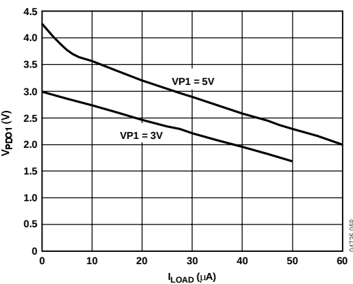
Figure 12. V PDO1 (Weak Pull-Up to VP) vs. I LOAD
