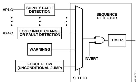
Figure 27. Sequence Detector Block Diagram
