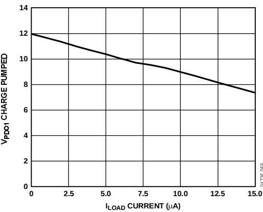
Figure 10. V PDO1 (FET Drive Mode) vs. I LOAD
