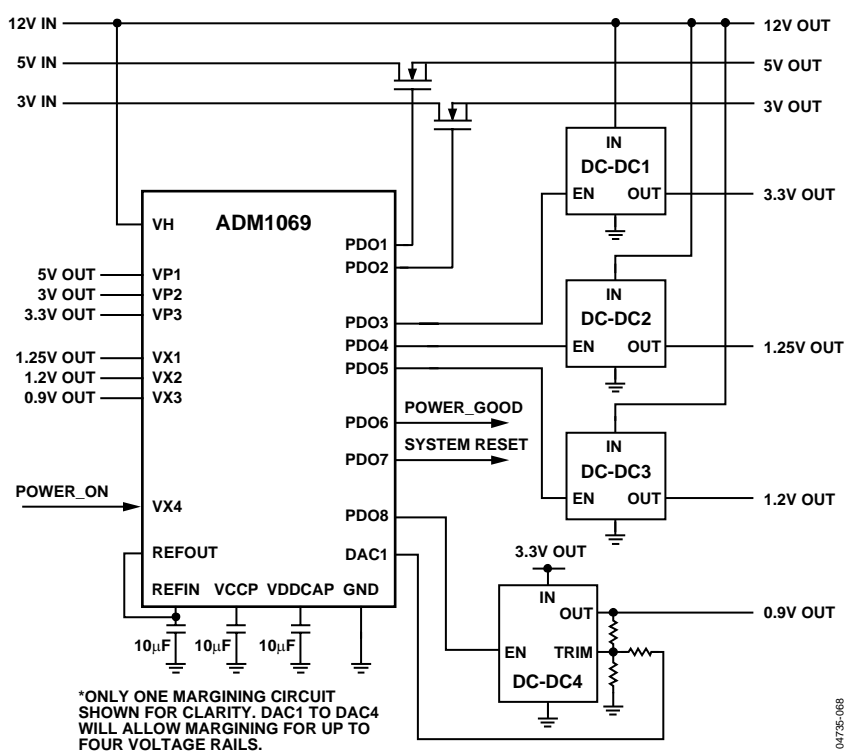
Figure 33. Applications Diagram
