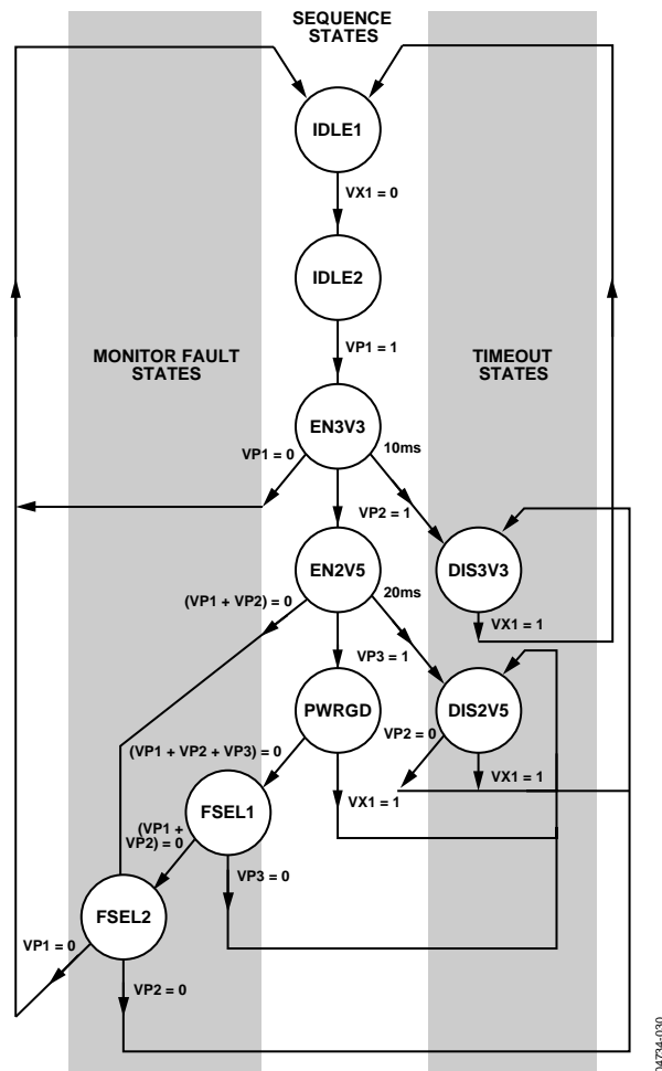
Figure 20. Sample Application Flow Diagram
