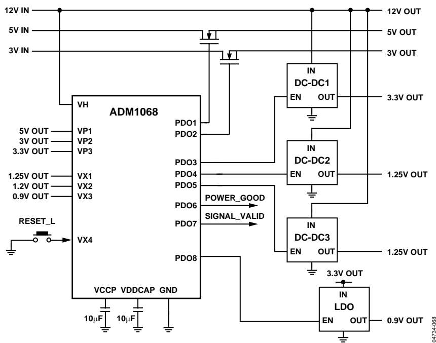
Figure 23. Applications Diagram
