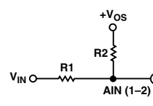
Figure 12. Scaling and Offsetting AIN(1-2) for Negative Inputs
