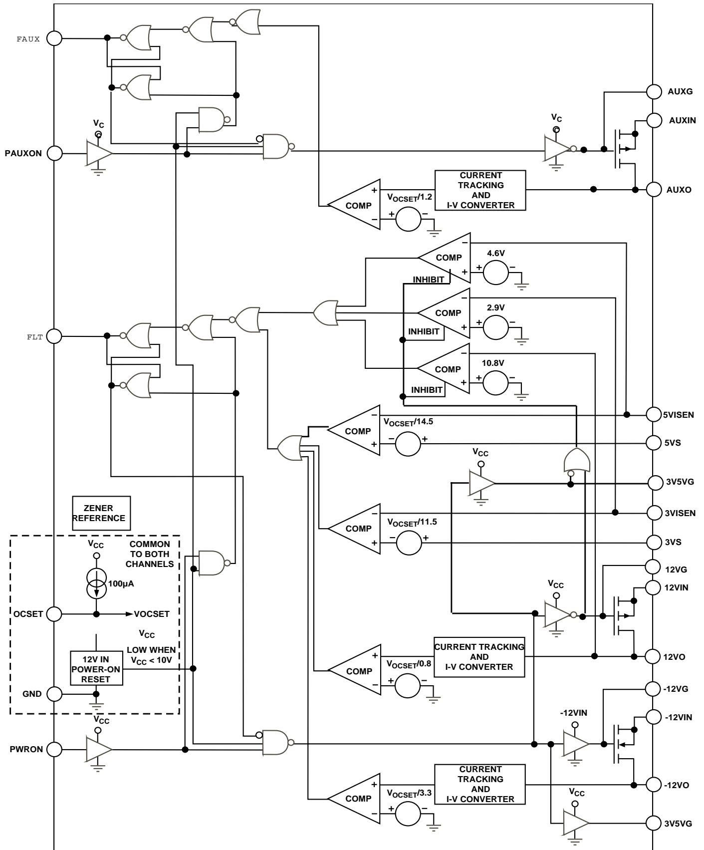
Figure 1. Simplified Schematic
