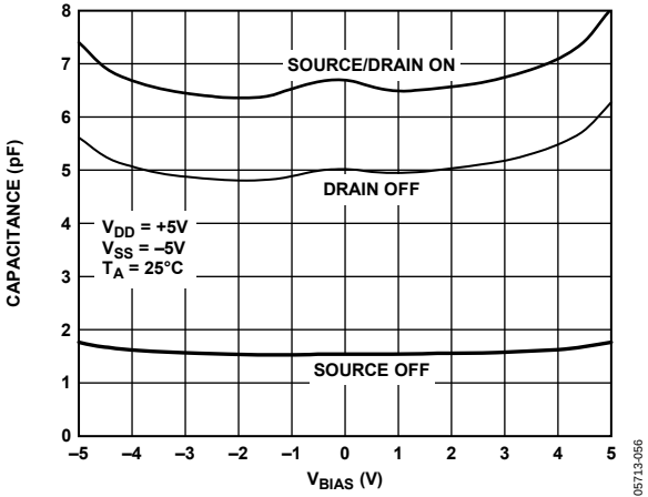
Figure 28. ADG1209 Capacitance vs. Source Voltage, ±5 V Dual Supply
