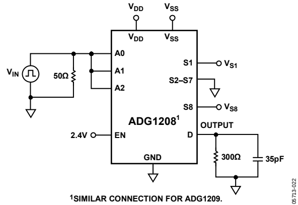
Figure 32. Address to Output Switching Times, t_{\text{TRANSITION}}
