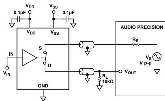
Figure 39. THD + Noise
