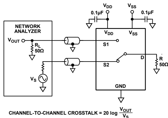
Figure 38. Channel-to-Channel Crosstalk
