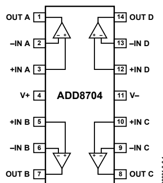
Figure 1. 14-Lead TSSOP (RU Suffix)
