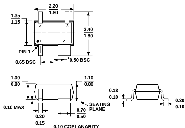
Figure 21. 4-Lead Thin Shrink Small Outline Transistor Package [SC70]
