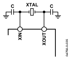
Figure 35. Crystal Connection
