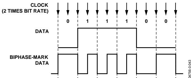
Figure 43. Biphase-Mark Encoding
