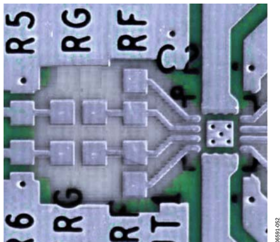
Figure 8. Ground and Power Plane Voiding in Vicinity of R_F and R_G
