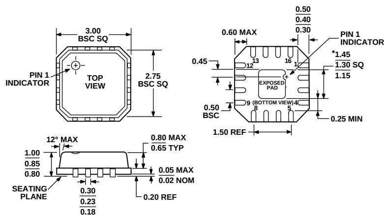
Figure 9. 16-Lead Lead Frame Chip Scale Package [LFCSP_VQ] 3 mm × 3 mm Body (CP-16-2)
