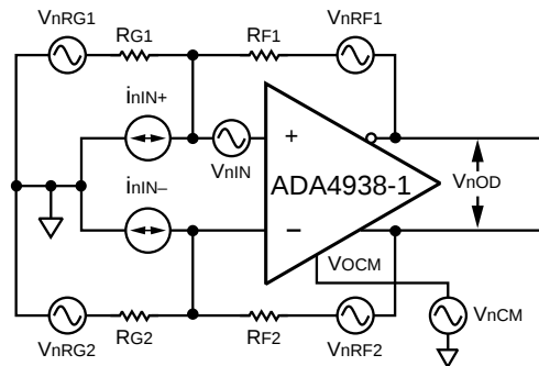
Figure 5. ADA4938-1 Noise Model
