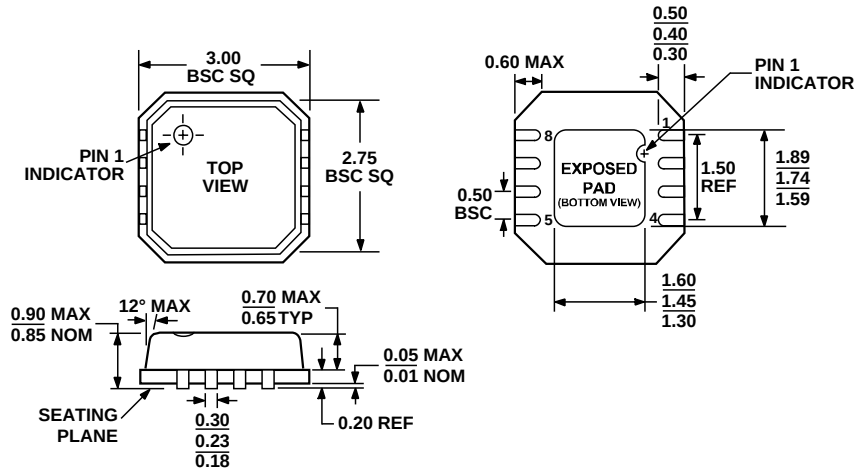
Figure 52. 8-Lead Lead Frame Chip Scale Package [LFCSP_VD] 3 mm × 3 mm Body, Very Thin, Dual Lead (CP-8-2)
