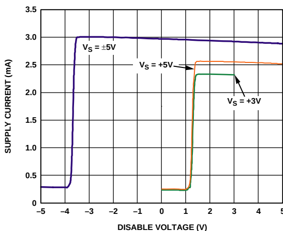
Figure 28. ADA4851-1, Supply Current vs. \overline{POWER\ DOWN} Pin Voltage
