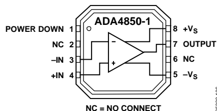
Figure 1. 8-Lead, 3 mm x 3 mm LFCSP
