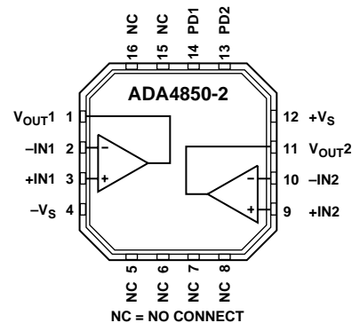
Figure 2. 16-Lead, 3 mm x 3 mm LFCSP
