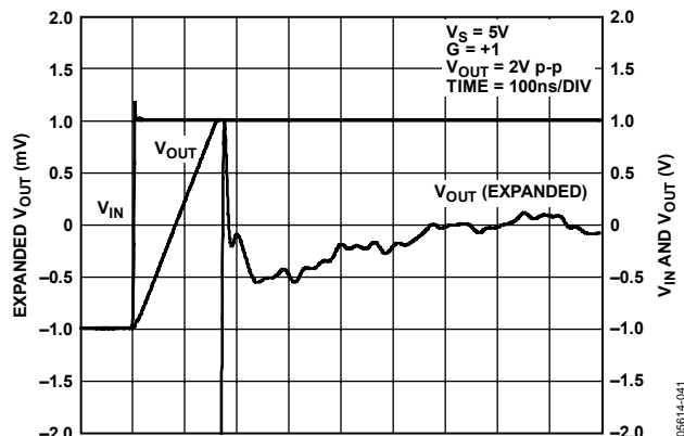
Figure 27. Settling Time
