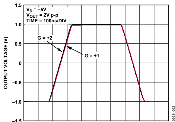
Figure 25. Large Signal Transient Response for Various Gains
