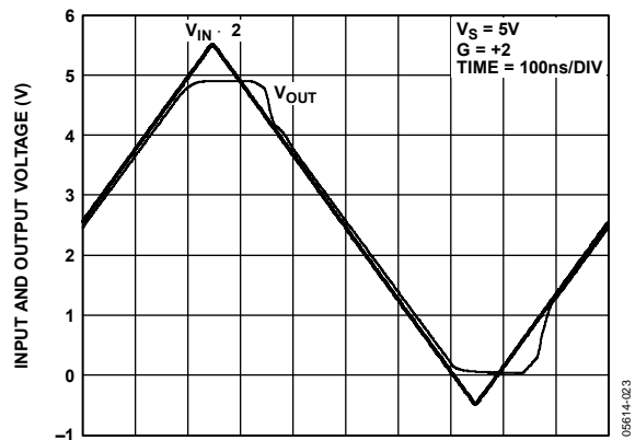
Figure 24. Output Overdrive Recovery
