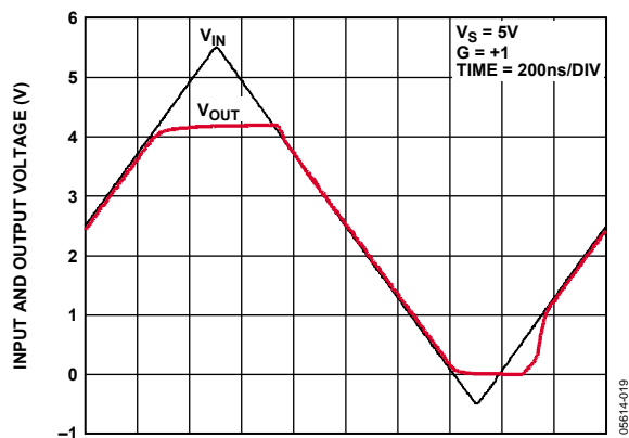
Figure 23. Input Overdrive Recovery
