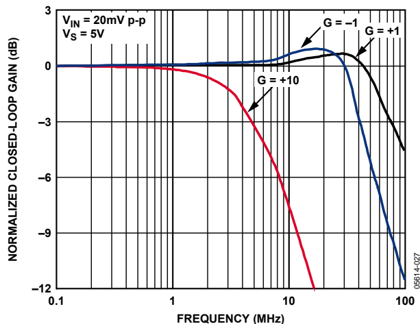
Figure 7. Small Signal Frequency Response vs. Gain
