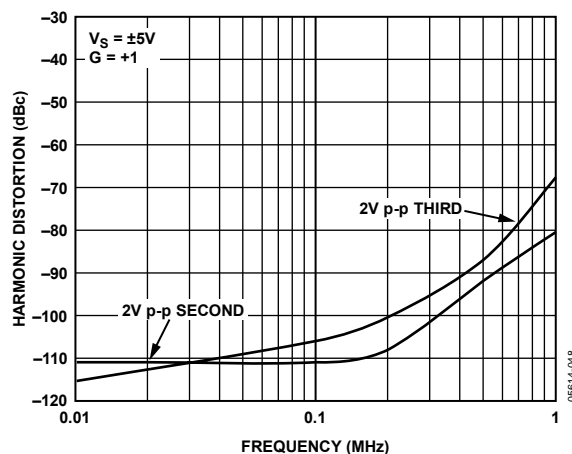
Figure 3. Harmonic Distortion
