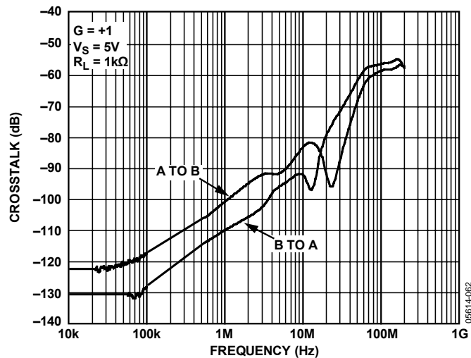
Figure 37. Crosstalk Output to Output
