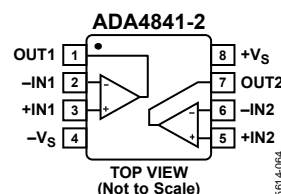
Figure 2. 8-Lead MSOP (RM-8)
