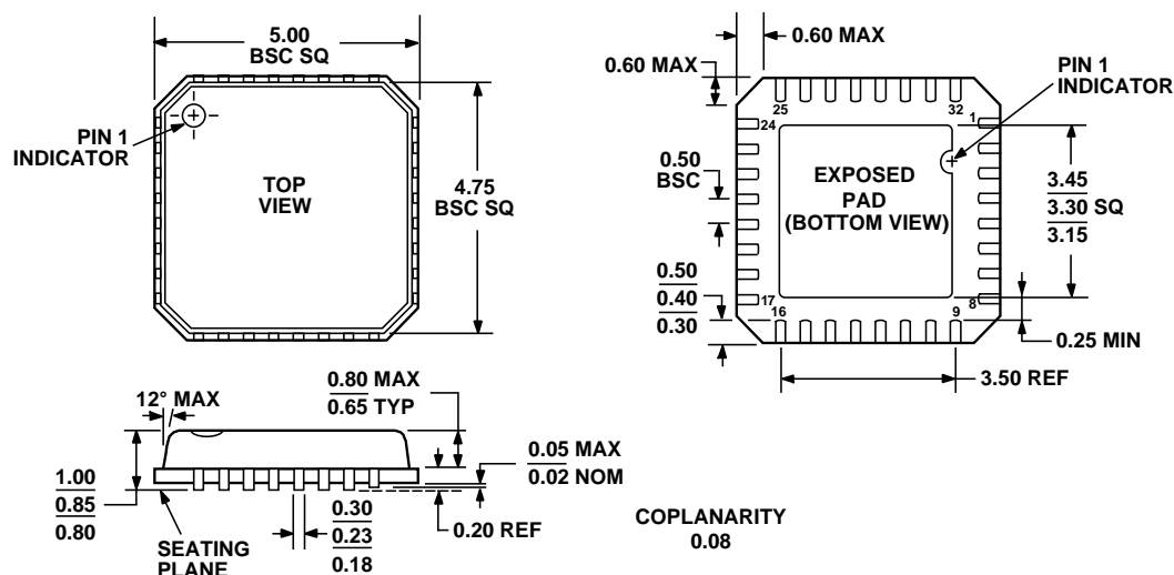
COMPLIANT TO JEDEC STANDARDS MO-220-VHHD-2 Figure 28. 32-Lead Lead Frame Chip Scale Package [LFCSP_VQ] 5 mm × 5 mm Body, Very Thin Quad (CP-32-3) Dimensions shown in millimeters
