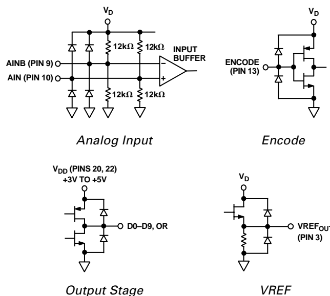
Figure 2. Equivalent Circuits
