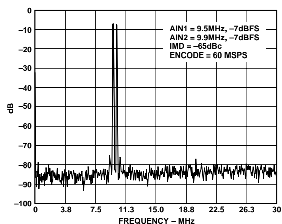
Figure 14. Two-Tone IMD
