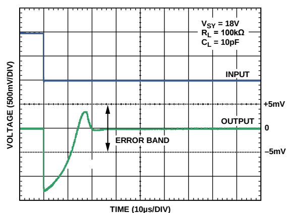
Figure 50. Negative Settling Time to 0.1%
