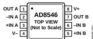
Figure 1. AD8546 (8-Lead MSOP)
