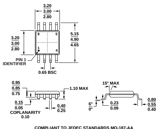
Figure 71. 8-Lead Mini Small Outline Package [MSOP] (RM-8)
