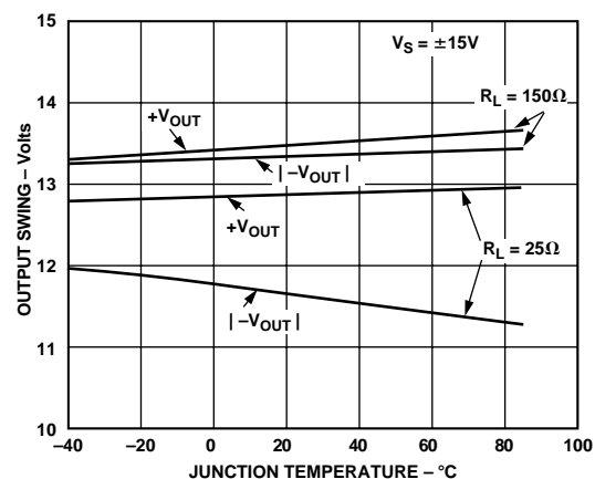
Figure 23. Single-Ended Output Swing vs. Temperature
