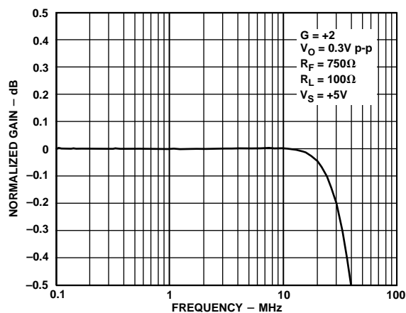
Figure 21. Gain Flatness; V_S = +5 V
