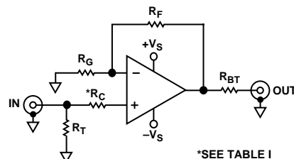
Noninverting Configuration
