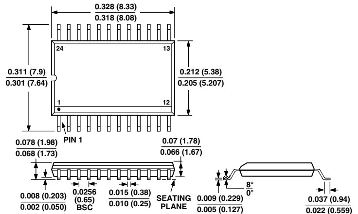
24-Lead Shrink Small Outline Package (RS-24)
