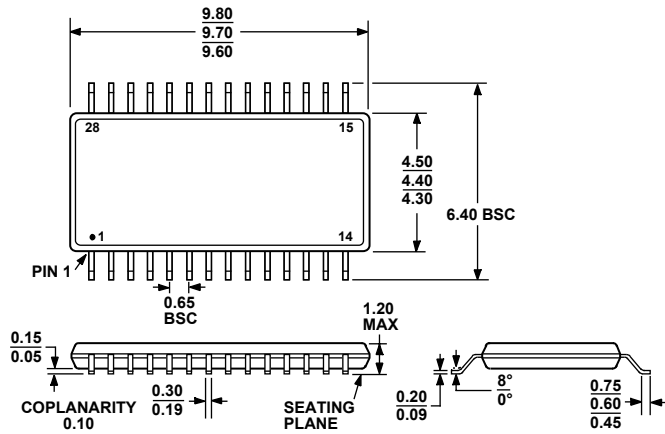
COMPLIANT TO JEDEC STANDARDS MO-153AE Figure 31. 28-Lead This Shrink Small Outline Package [TSSOP] (RU-28)—Dimensions shown in millimeters
