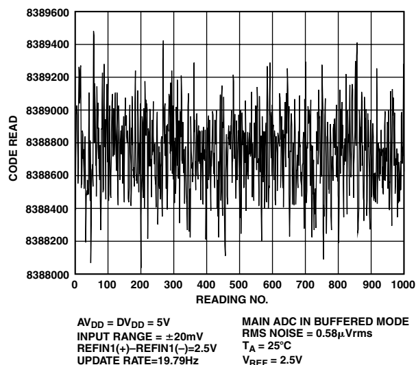
TPC 1. Typical Noise Plot on \pm 20\ mV Input Range with 19.79 Hz Update Rate
