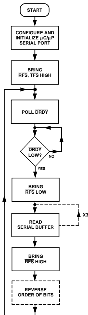
Figure 15. Flowchart for Continuous Read Operations to the AD7711
