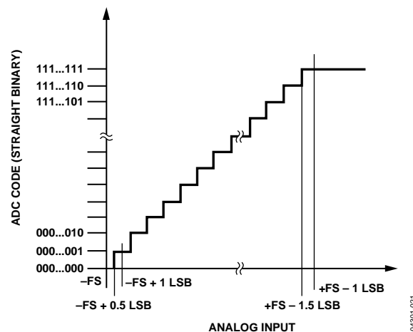
Figure 21. ADC Ideal Transfer Function
