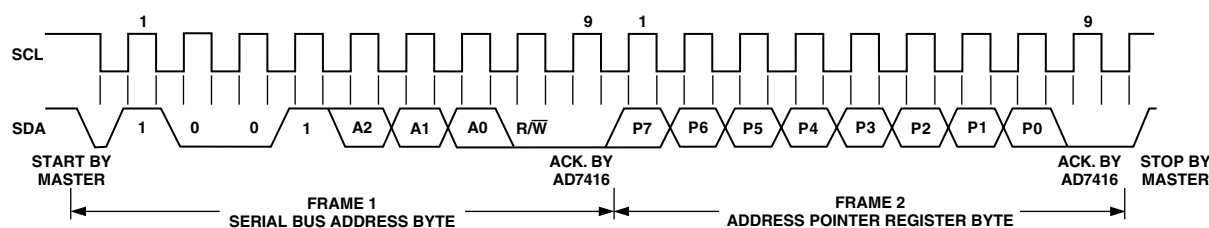
Figure 8. Writing to the Address Pointer Register to Select a Data Register for a Subsequent Read Operation
