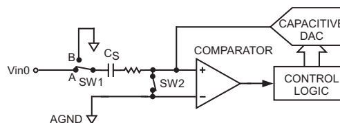
Figure 4. ADC Acquisition Phase(Single Ended)
