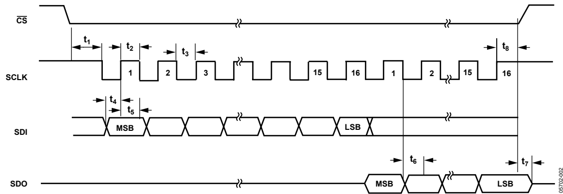
Figure 3. SPI Detailed Timing Diagram
