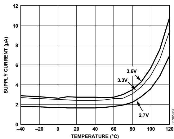
Figure 15. Shutdown Supply Current vs. Temperature (Supply Current = I_{CC} + D I_{CC} )
