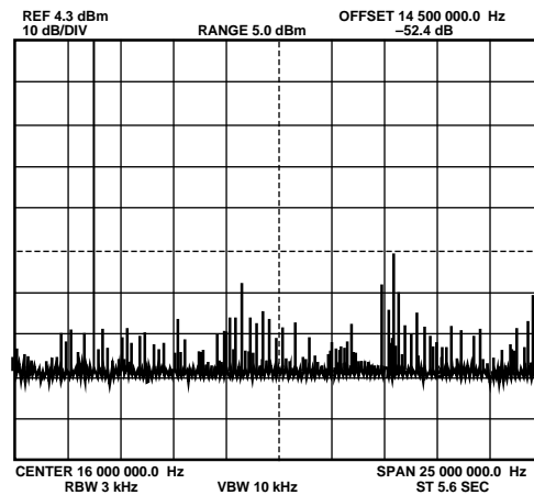
Figure 26. f_{CLK} = 50\text{ MHz} , f_{OUT} = 7.1\text{ MHz}
