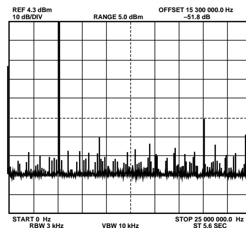
Figure 28. f_{CLK} = 50\text{ MHz} , f_{OUT} = 5.1\text{ MHz}
