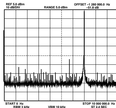
Figure 27. f_{CLK} = 20\text{ MHz} , f_{OUT} = 7.1\text{ MHz}
