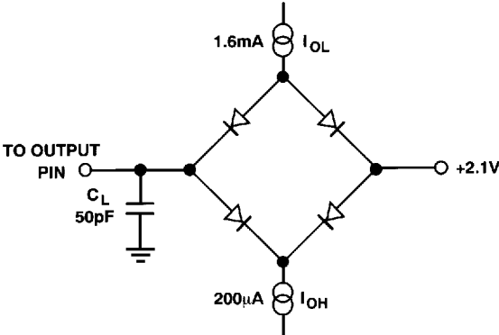
Figure 2. Load Circuit for Access Time Test
