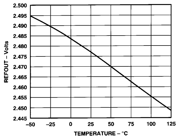
Figure 19. Typical Plot of Reference Variation vs. Temperature
