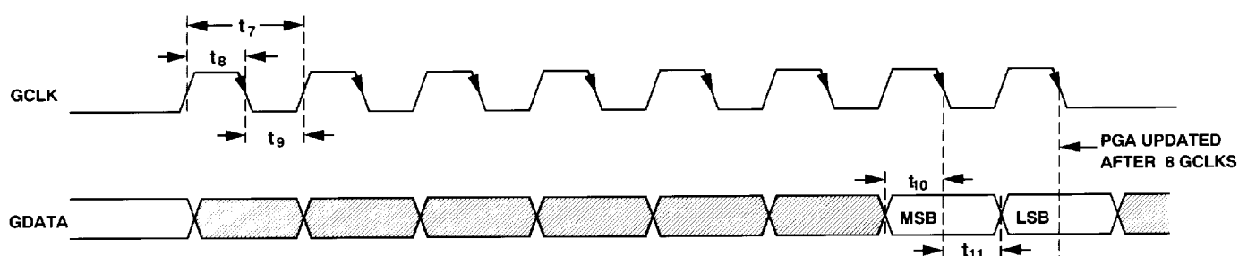
Figure 4. PGA Timing Diagram
