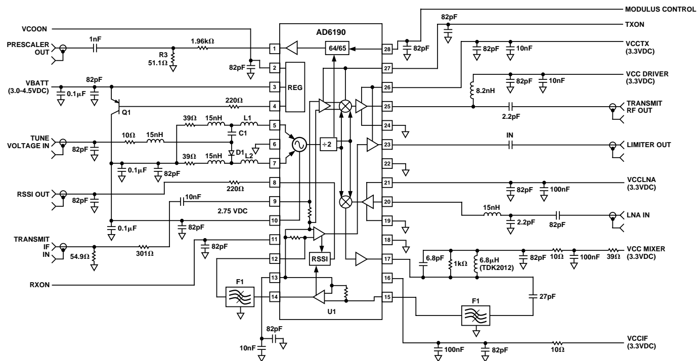
Figure 1. Test Circuit
